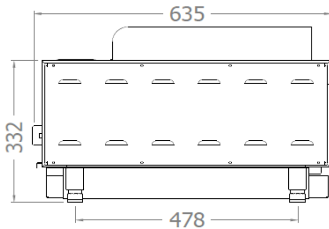
IS 1 / IS 2 / IS 3 / IS 4 Vue de profil
